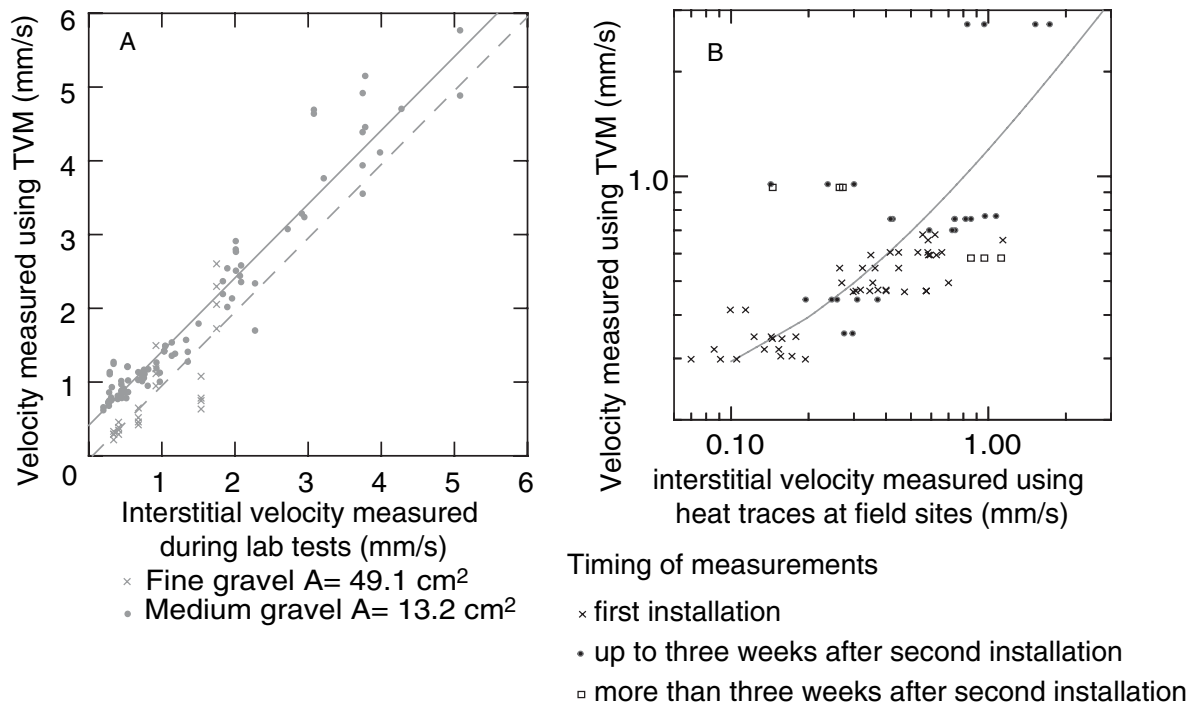
Figure 6. Calibration data for TVM output against in-situ heat trace measurements of interstitial flow rate. Calibration procedures discussed in text. (A) Laboratory calibration data for two different gravels. (B) Best-fit field calibration across all study sites
