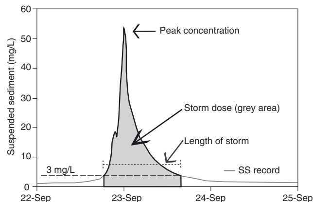
Figure 3. Typical suspended sediment (SS) record for a runoff event with definition of integrated suspended sediment dose for the event (area under curve in \text{mg l}^{-1} \text{day}^{-1} ). Between-event background concentration was approximately 1 \text{ mg l}^{-1} .
