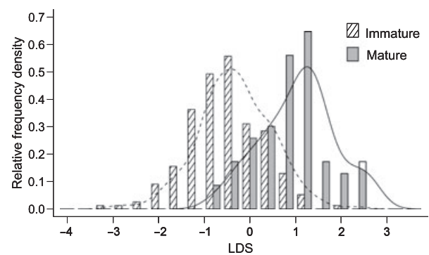
Fig. 4 Canonical scores from the discriminant function used to classify mature and immature individuals. The broken line traces the relative frequency distribution of the canonical scores of individuals captured in rapid habitats whereas the continuous line traces scores in slow water habitats.
